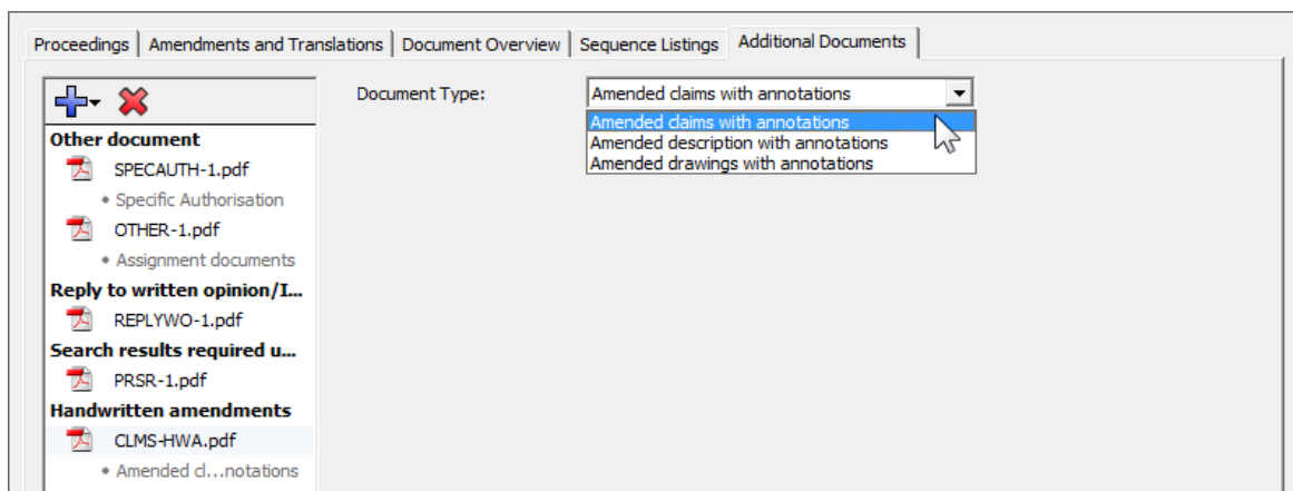
Figure 232: Document with handwritten amendments attached
