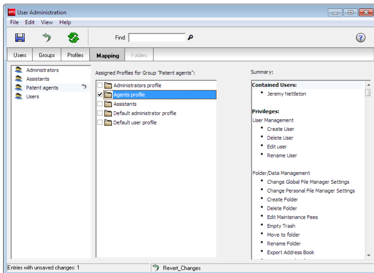
Figure 86: Check privileges after mapping profiles to groups
