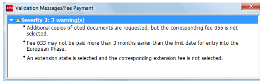
Figure 239: Validation messages with information on the fees to be paid
