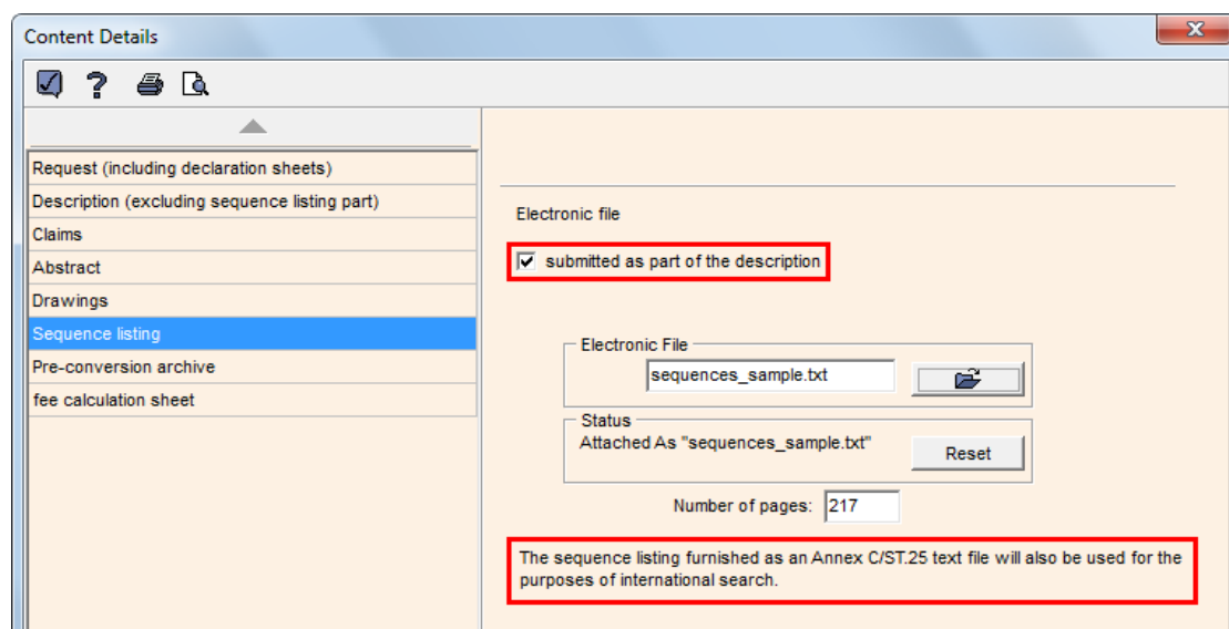
Figure 391: The sequence listing submitted as part of the description in APP or TXT format will also be used for the purposes of the international search
