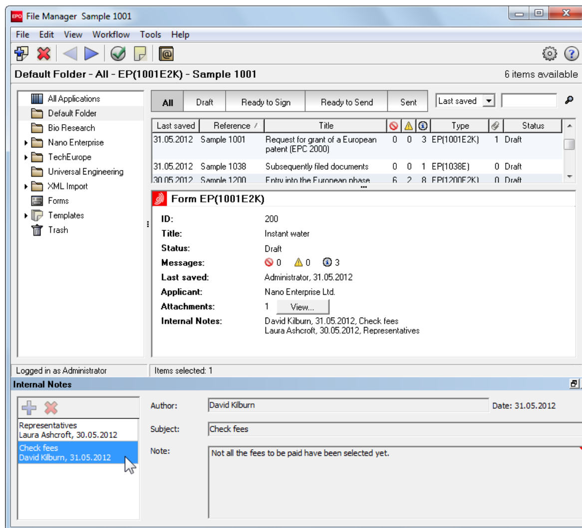
Figure 37: Example of an internal note in the docked Internal Notes window in File Manager
