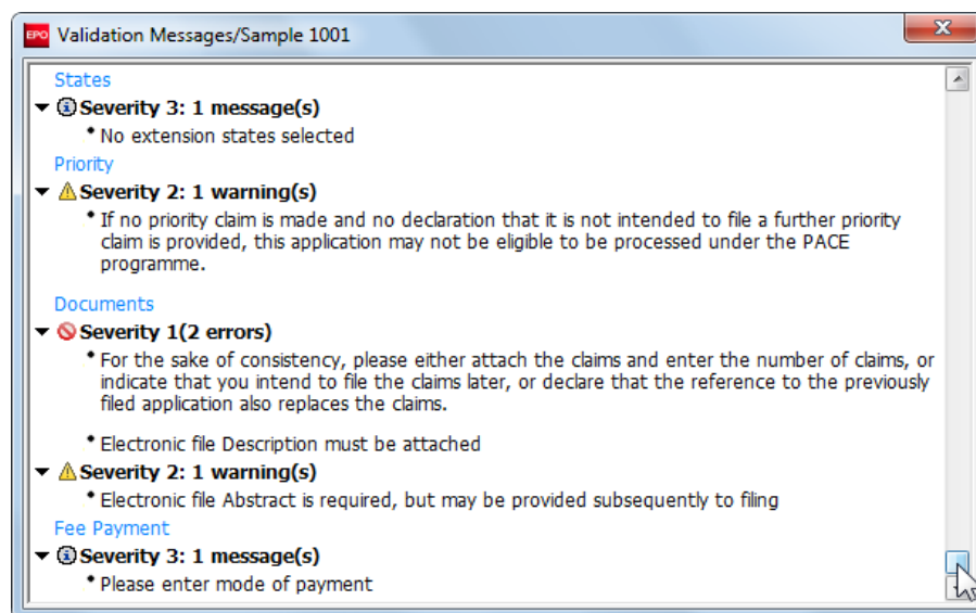
Figure 35: All validation messages for an application
