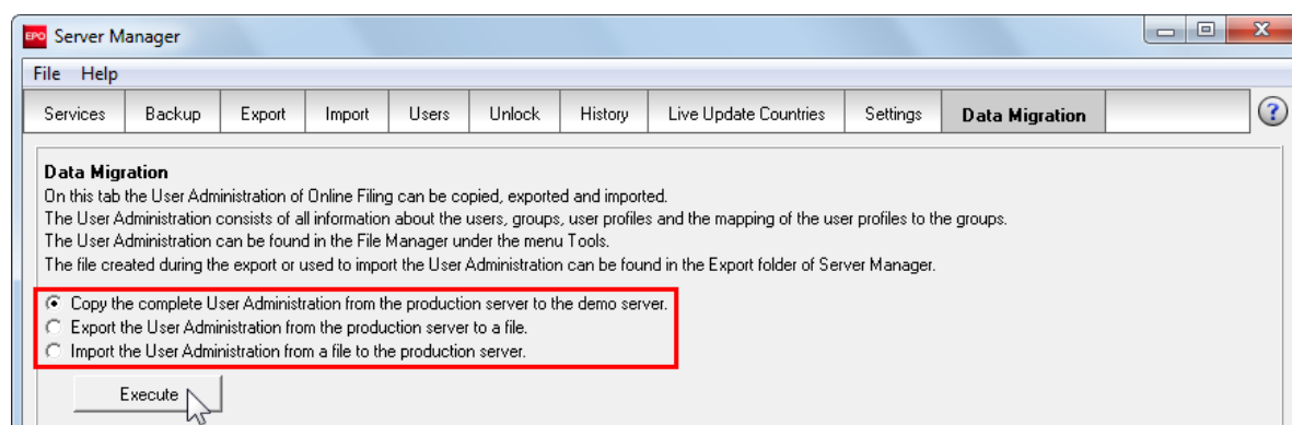
Figure 467: Options for migrating the User Administration
