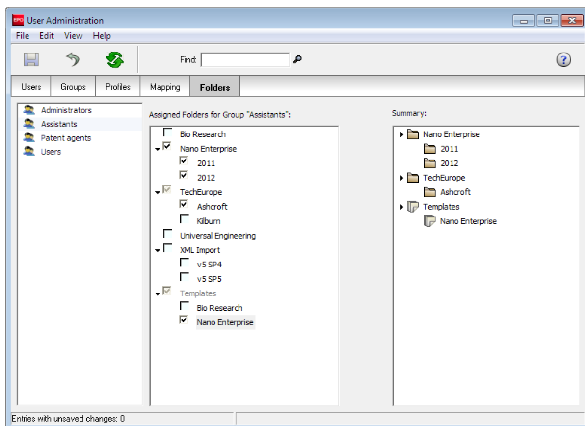
Figure 87: Enabling folders for a group
